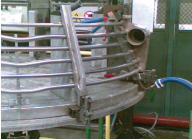
Liquid tubing brazing
