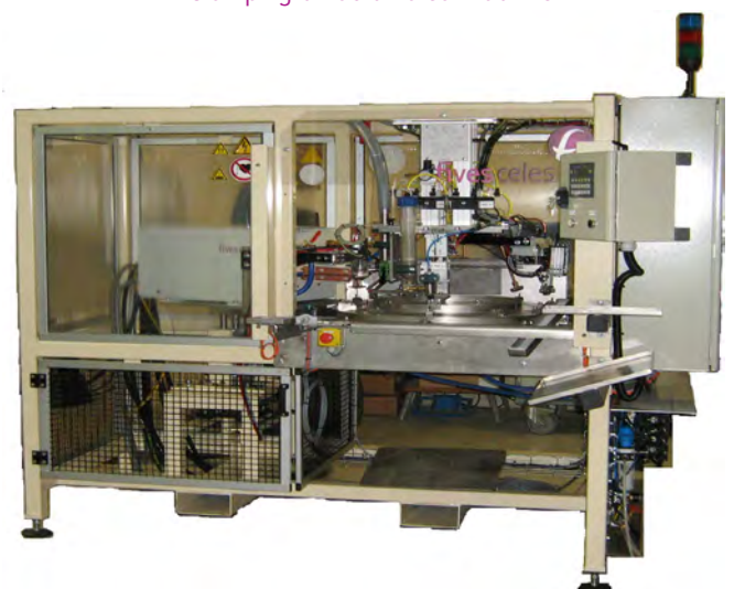
Brazing of electrical contacts on a machine automated carousel
