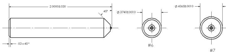
Dimensions shown for 2" shank length and diameter styles 6 and 7
