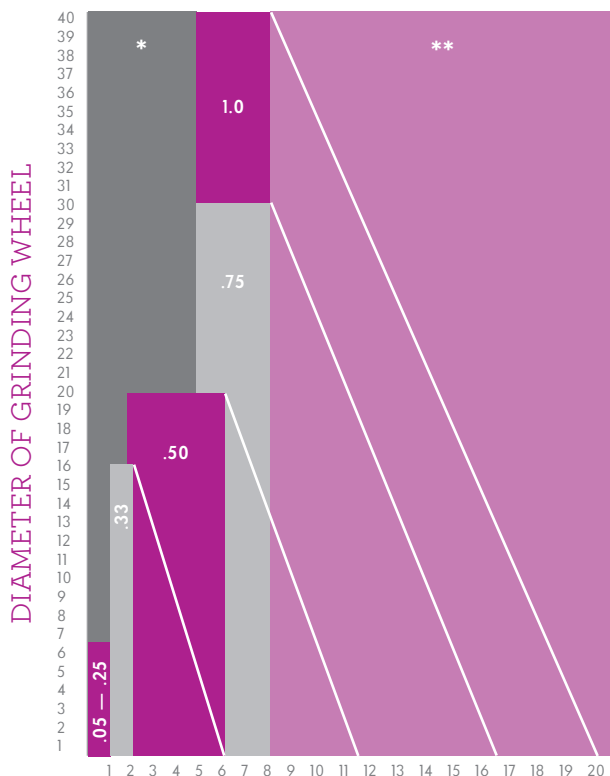
Dimensions shown for 2" shank length and diameter styles 6 and 7
