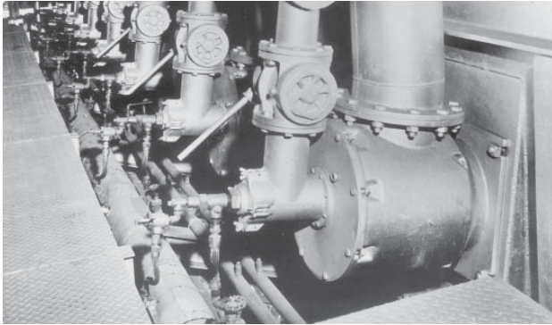
5642 Atomizers firing heavy oil in Dual-Fuel™ burners on a steel mill reheat furnace.
