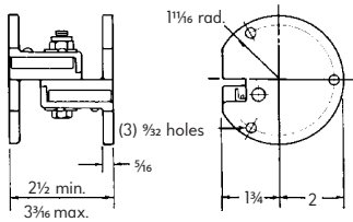
4-3159-1 Expansion Ignition Coupling
