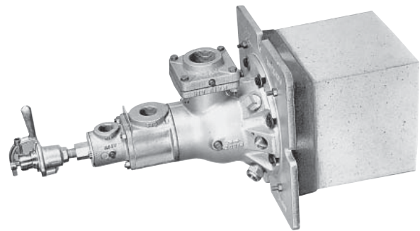
6425 Burner Complete shown with optional (recommended) Sensitrol Oil Valve.
