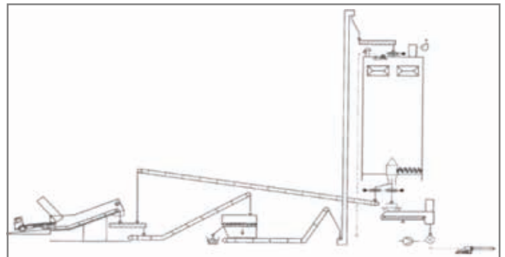
Semi-dry and dry line burner feeding
